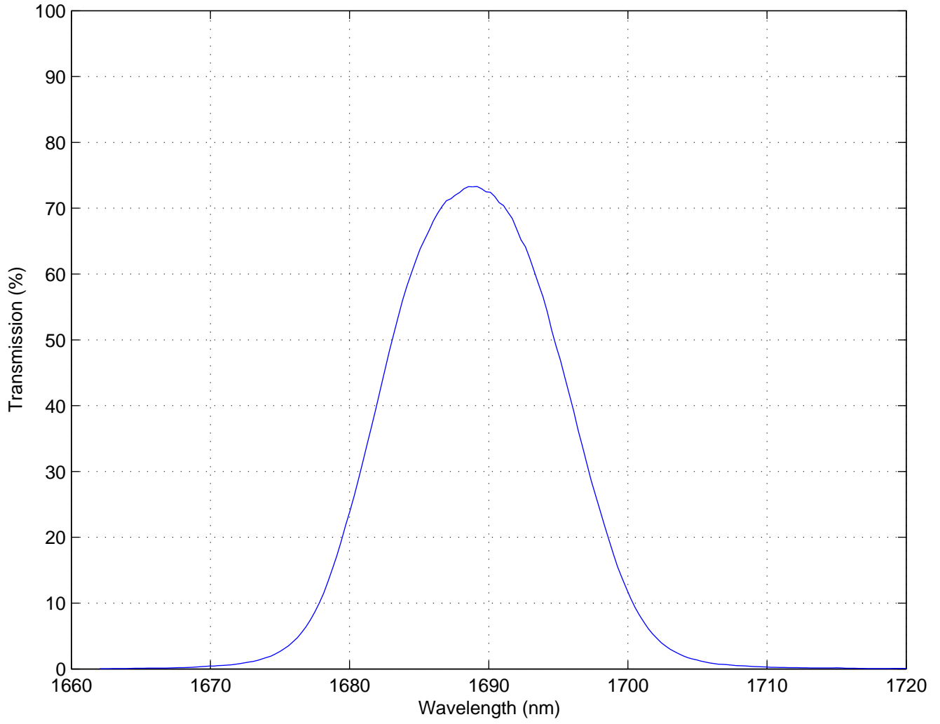
Filter #228, Fell-continuum, vacuum wavelength, T=74K
