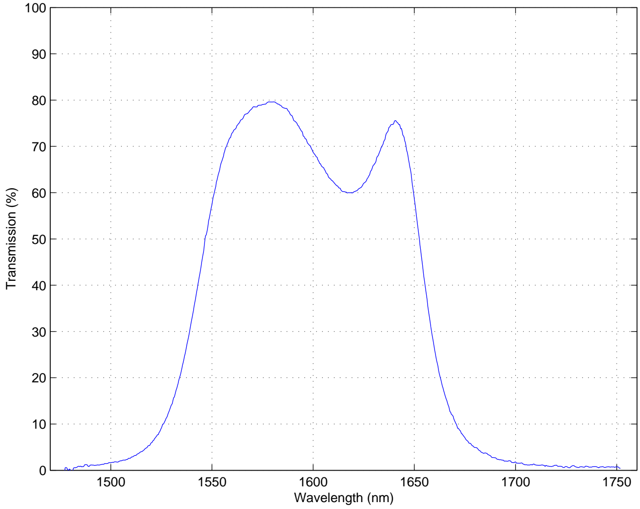
Filter #223, CH4 s, vacuum wavelength, T=74K
