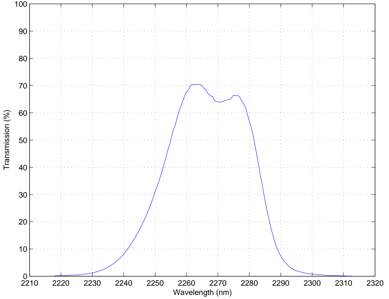
Filter #210, K-continuum, vacuum wavelength, T=74K
